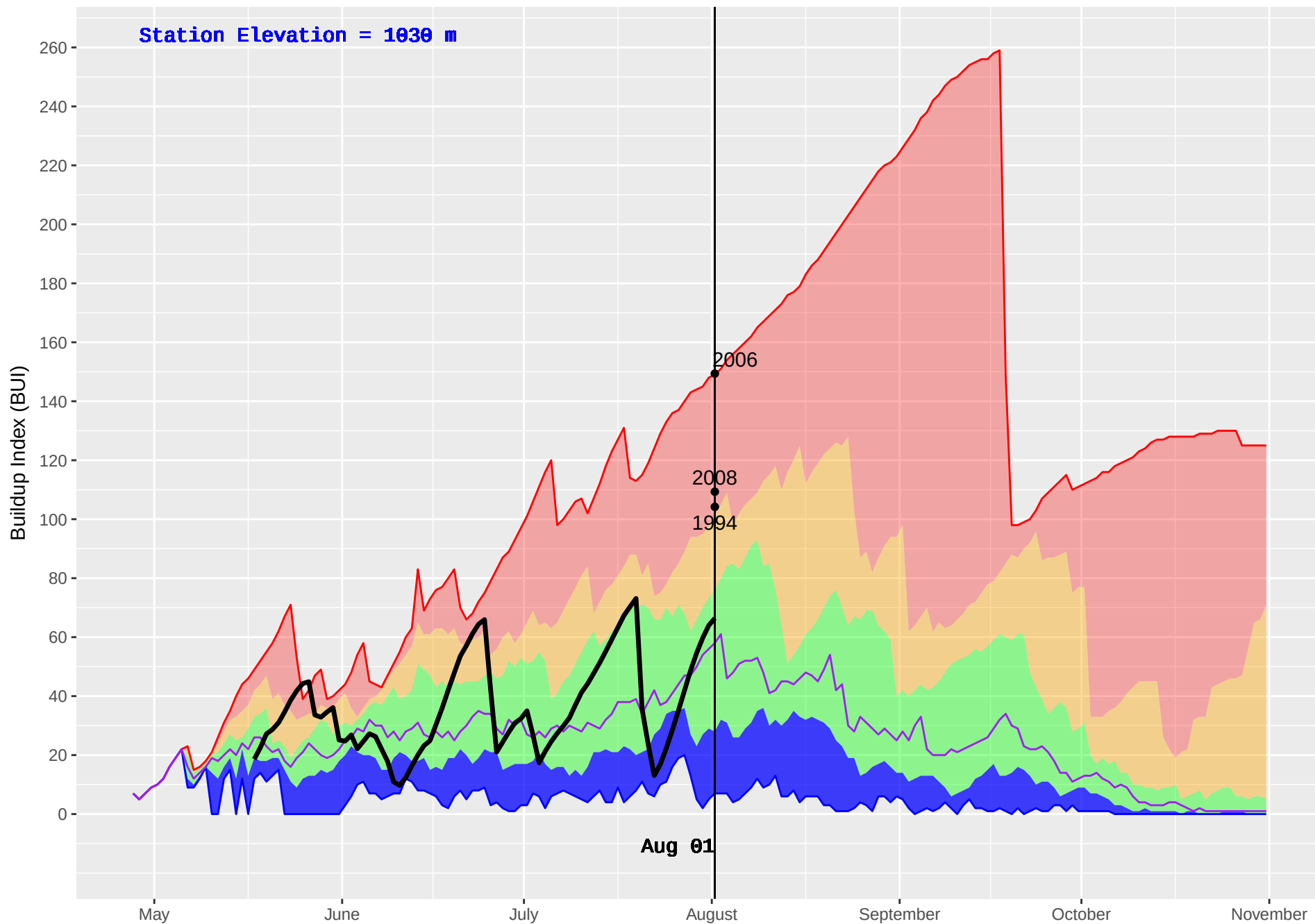
WITCH (154) : Historical (1993–2016) and Current (2018) Daily Buildup Index (BUI)
