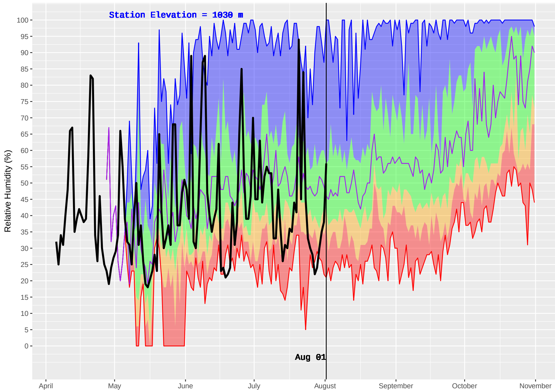
WITCH (154) : Historical (1993–2016) and Current (2018) Daily Relative Humidity
