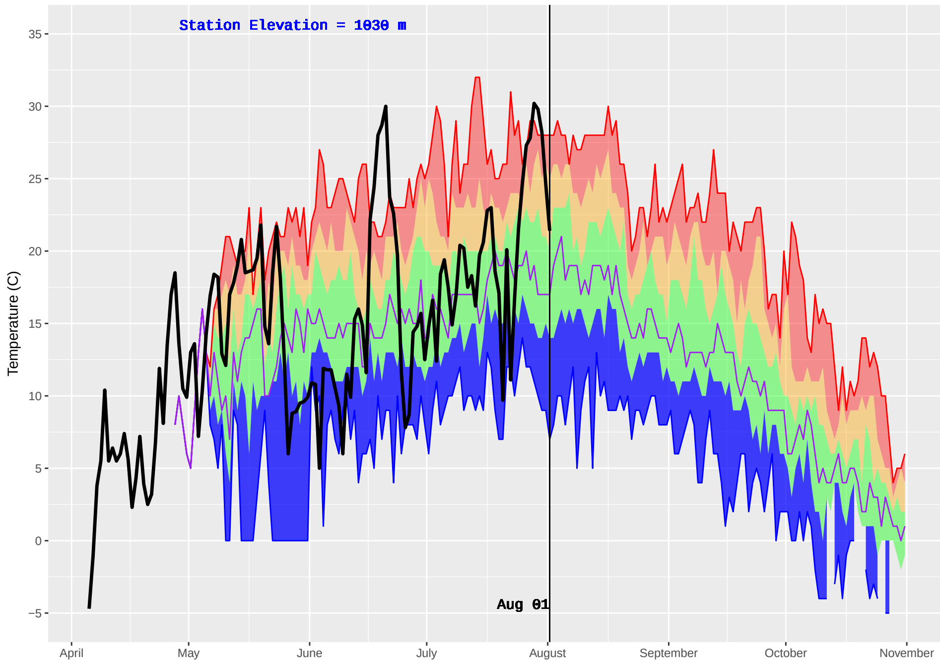
WITCH (154) : Historical (1993–2016) and Current (2018) Daily Temperature
