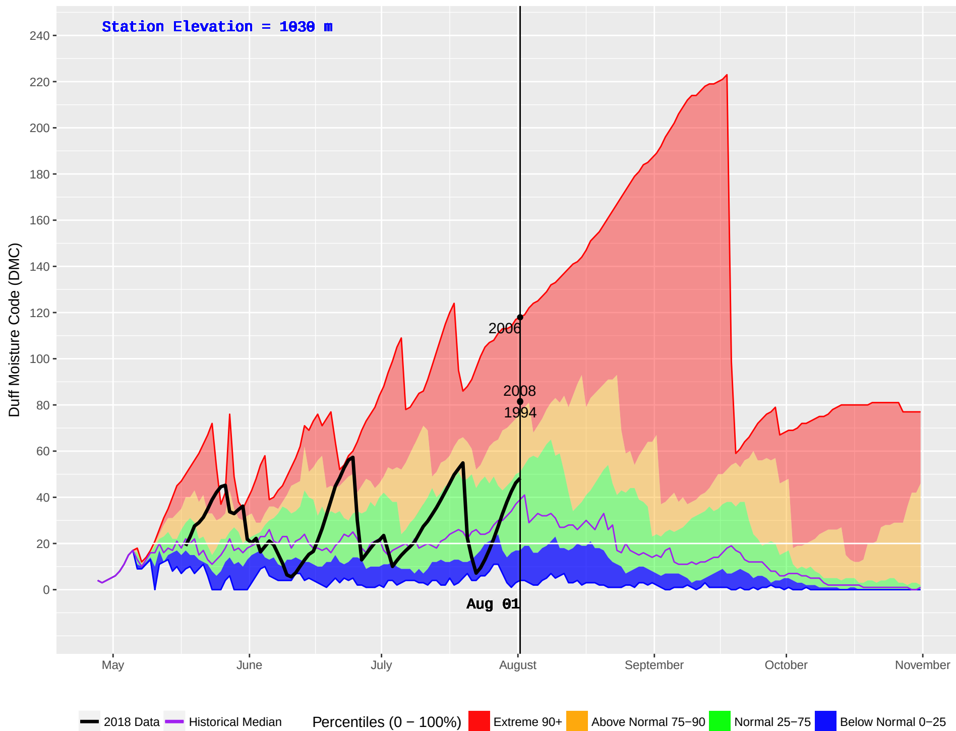
WITCH (154) : Historical (1993–2016) and Current (2018) Daily Duff Moisture Code (DMC)
